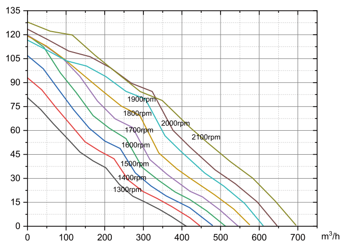
NEC6115R200 (5 Blades) \phi 200 mm Plastic Pa
